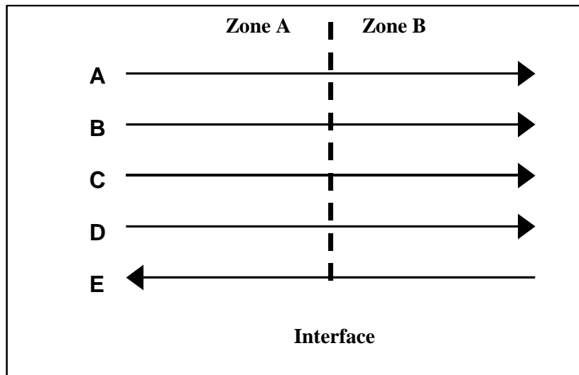
Figure 6: Transaction Example
